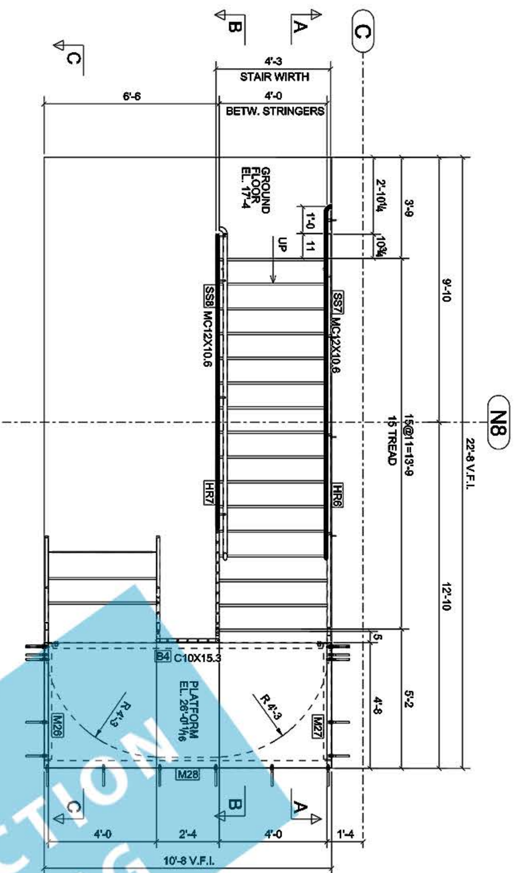
PLAN @GROUND LEVEL
