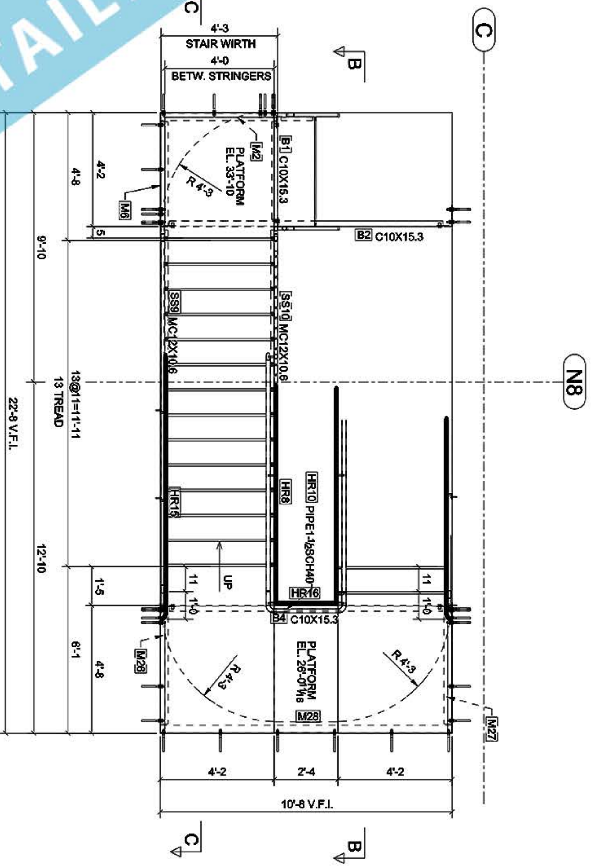
PLAN @PLATFORMS
